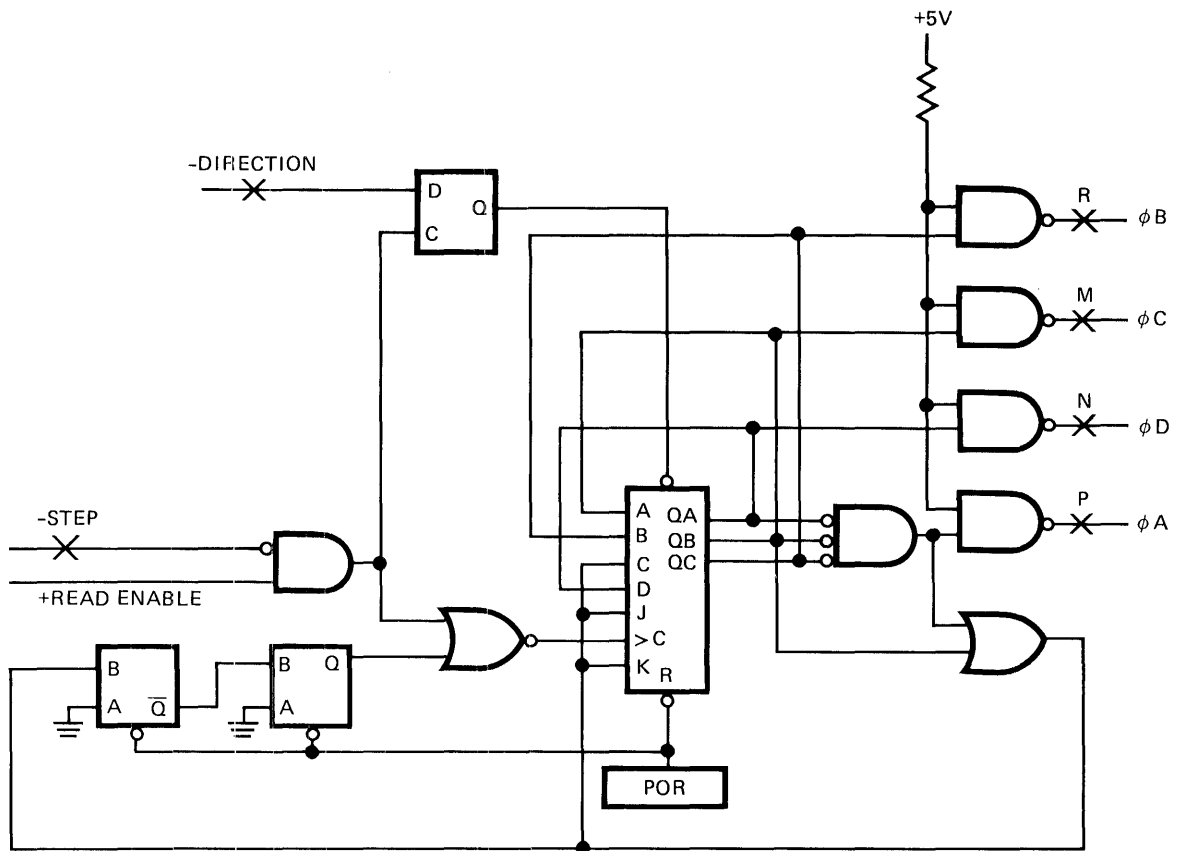
FIGURE 15. STEPPER CONTROL FUNCTION DIAGRAM
