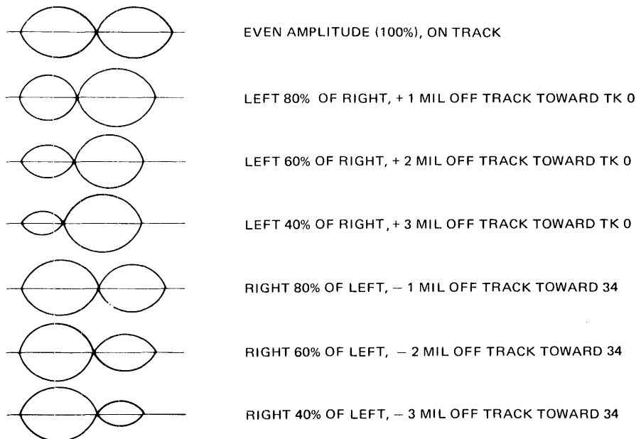
FIGURE 12. HEAD RADIAL ALIGNMENT
